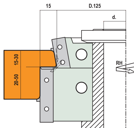
PROFILO INTERNO VETRO INTERNAL PROFILE SASH
