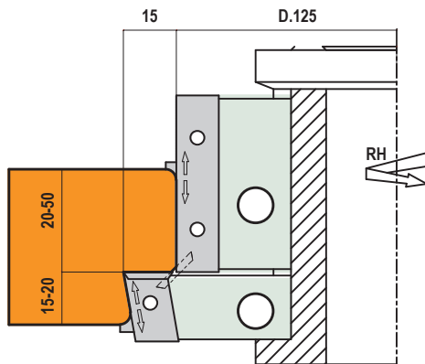
CONTROSAGOMA INTERNO VETRO SASH COUNTERPROFILE
