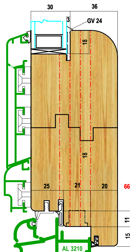
PORTA BALCONE
