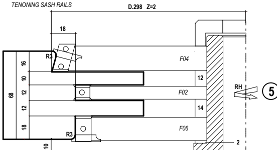
TANONI TRAVERSI ANTA TENONING SASH RAILS
