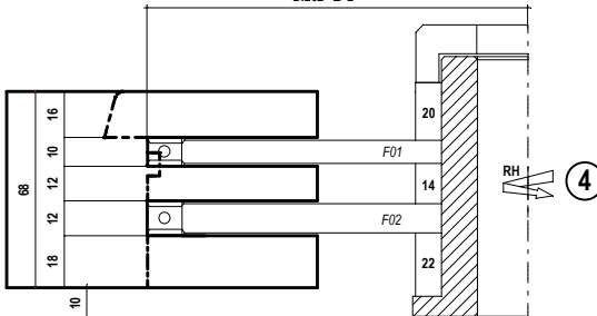
TENONI MONTANTI ANTA TENONING SASH JAMBS
